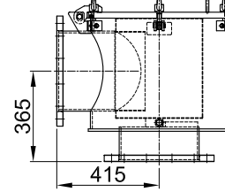
DN 300
