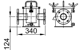
DN 150
