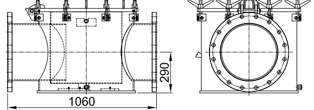
DN 400
